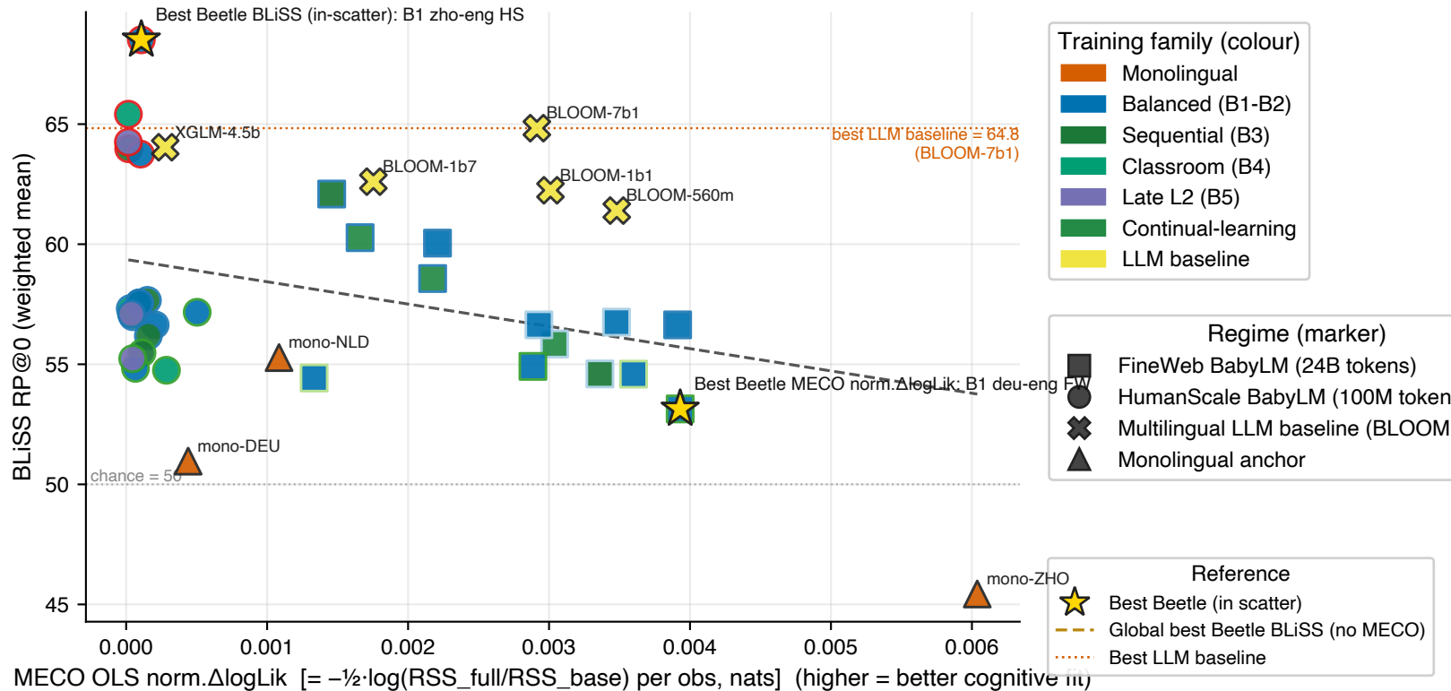
BLiSS vs MECO norm. \Delta\log\text{Lik} — final checkpoint, one point per model ( \rho=-0.33 , r=-0.34 , n=41 )
